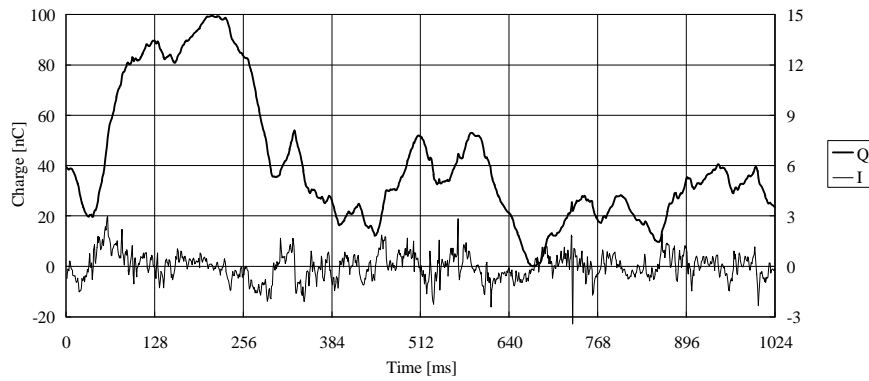
Figure 1 : Surface charge on sensor and displacement current from sensor
