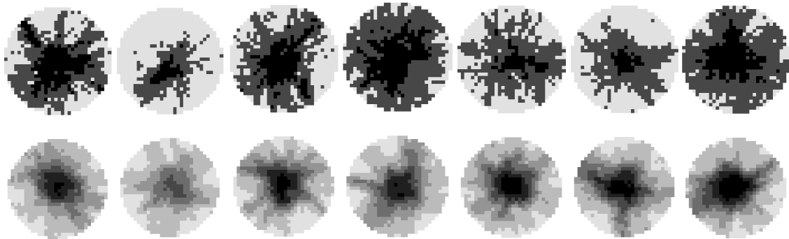
Figure 3 : Image at the bottom of riser in low solid load, G_s = 40.0[\text{kg}/\text{m}^2\text{s}] , Gas velocity = 8.5[m/s] (upper = displacement current, lower = charge)
