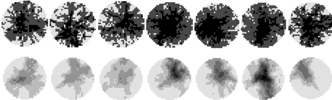
Figure 4 : Image at the bottom of riser in high solid load, G_s = 59.1[\text{kg}/\text{m}^2\text{s}] , Gas velocity = 7.3[m/s] (upper = displacement current, lower = charge)
