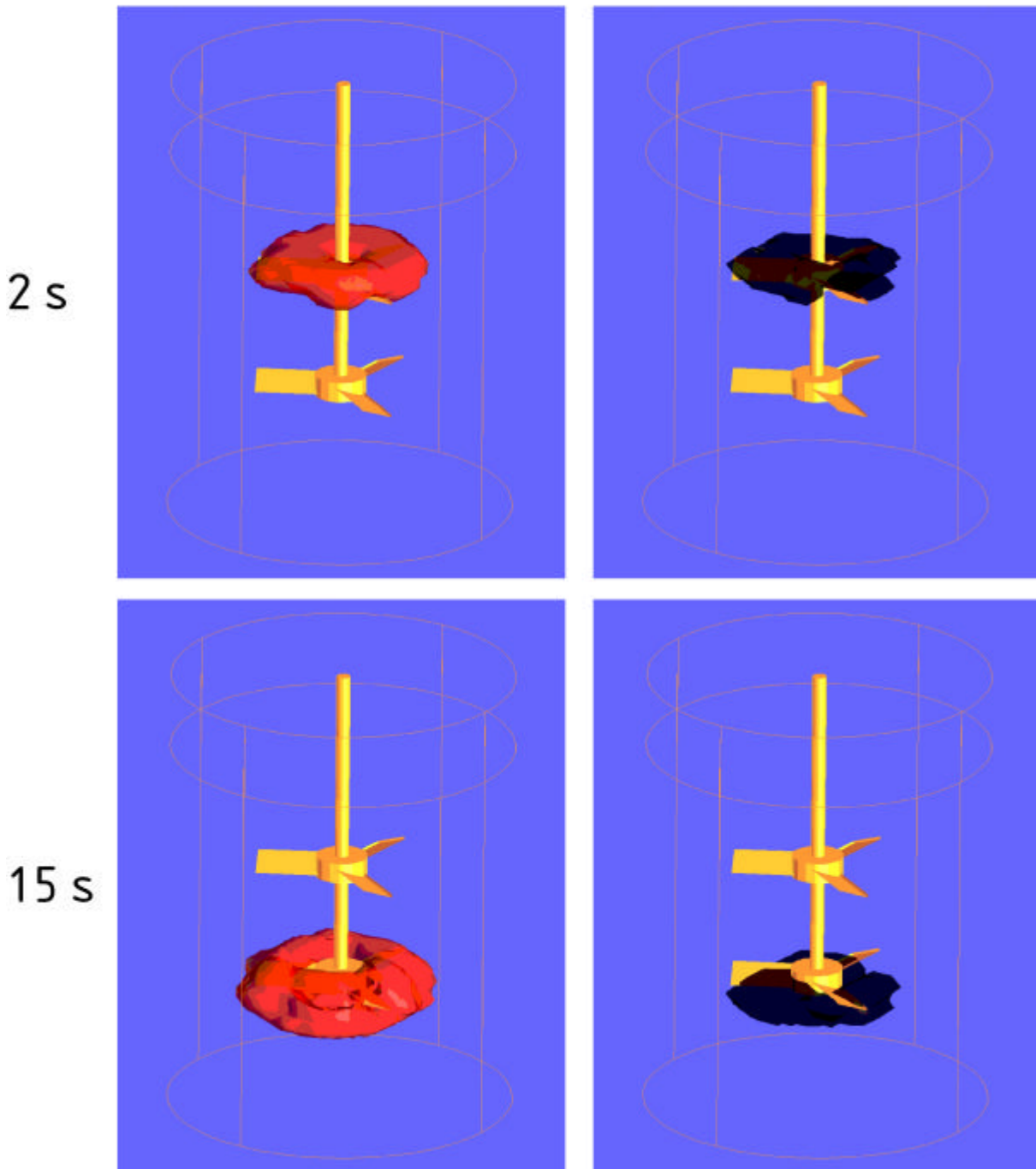
Figure 5: Mixing with the combination of the two Pitched Blade Impellers
