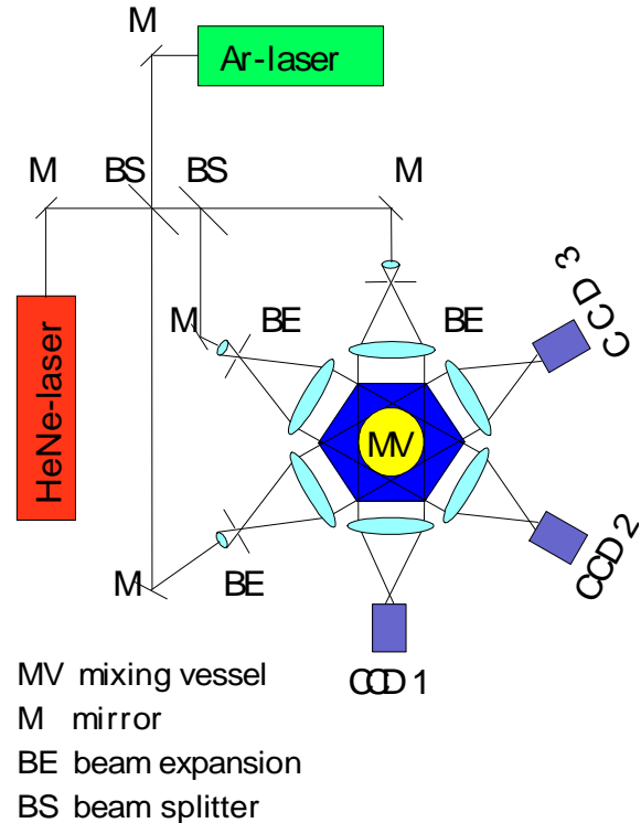
Figure 2: Optical Setup for the tomographical dual wavelength photometry.
