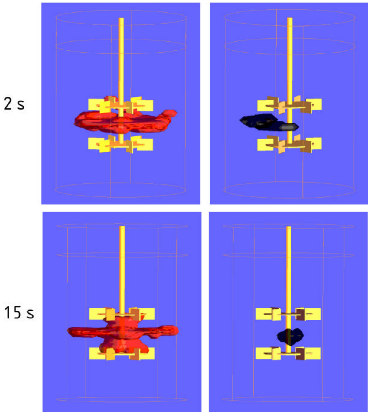
Figure 6: Mixing with the combination of the two Rushton turbines
