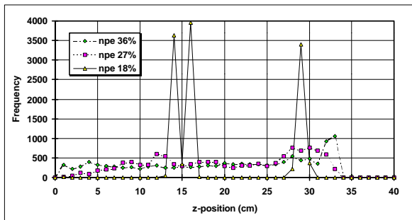
Figure 10: Axial position profiles for a series of experiments using narrow particle size distribution polyethylene.
