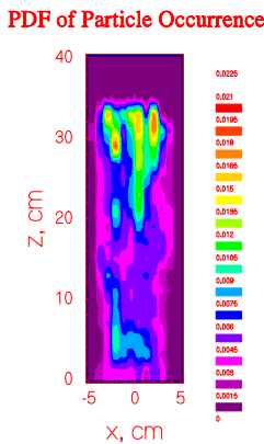
Figure 4: Probability distribution function (PDF) of particle occurrence in the bed
