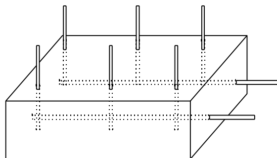
Figure 2: Schematic of the physical model used in the porous media displacement experiments
