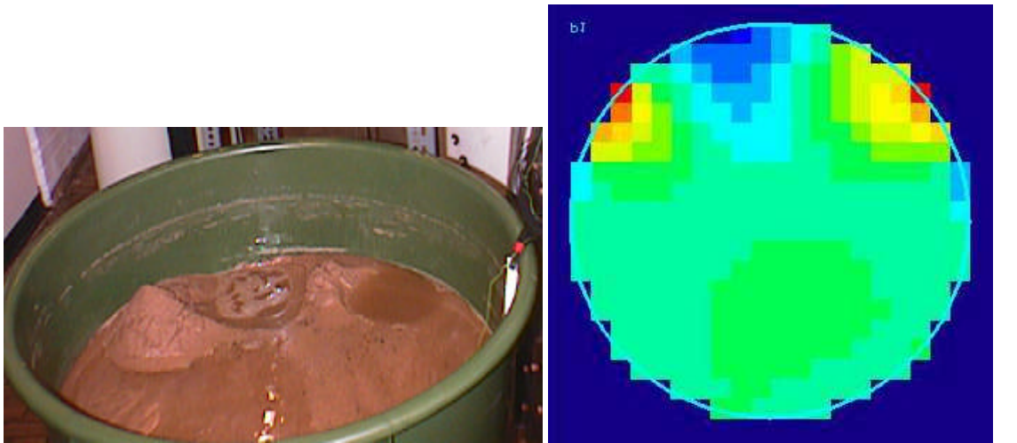
Figure 6 On-line detection of 2 large depressions in a sand filter cake
