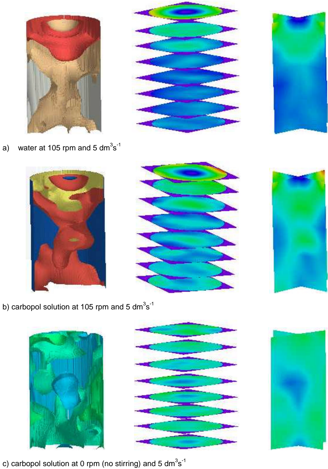
Figure 2 Tomography of gas-liquid mixing
