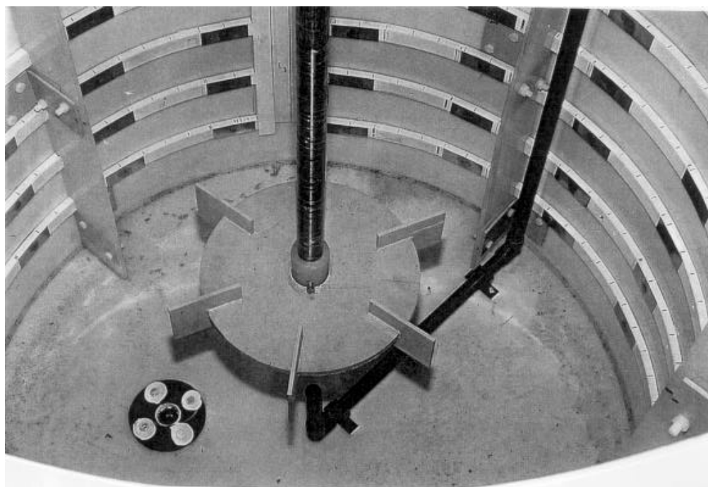
Fig.1 Set of 8x16 element sensing rings installed in 1.5 m stirred vessel
