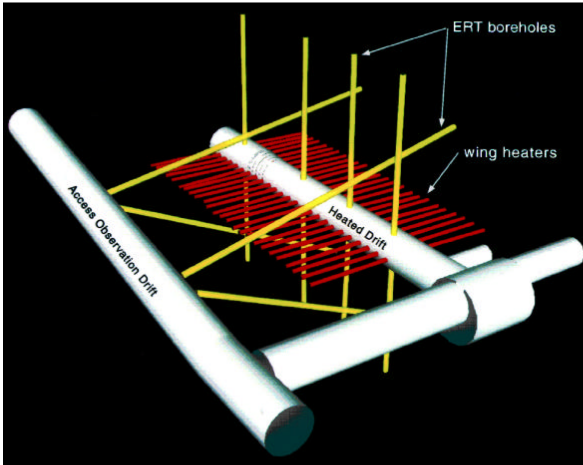
Figure 1: The Drift Scale Test layout in the Exploratory Studies Facility. A thermal bulkhead isolates the 47.5 m heated drift from the connecting drift and the access observation drift. The 12 boreholes used for ERT are also shown, 8 drilled from the heater drift and 4 drilled from the access observation drift.
